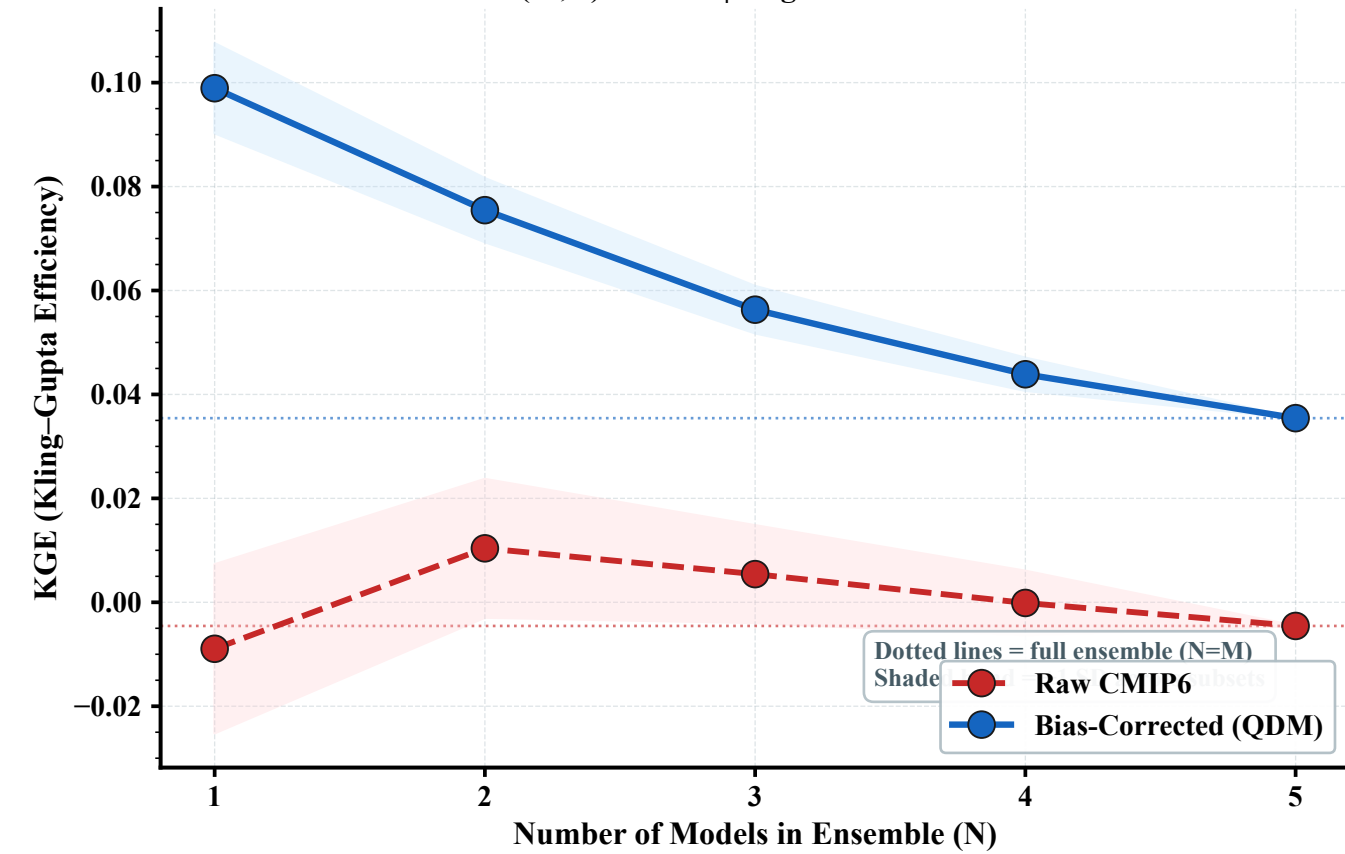
(a) KGE (Kling–Gupta Efficiency) Mean \pm SD across all C(M,N) subsets | Higher = better
