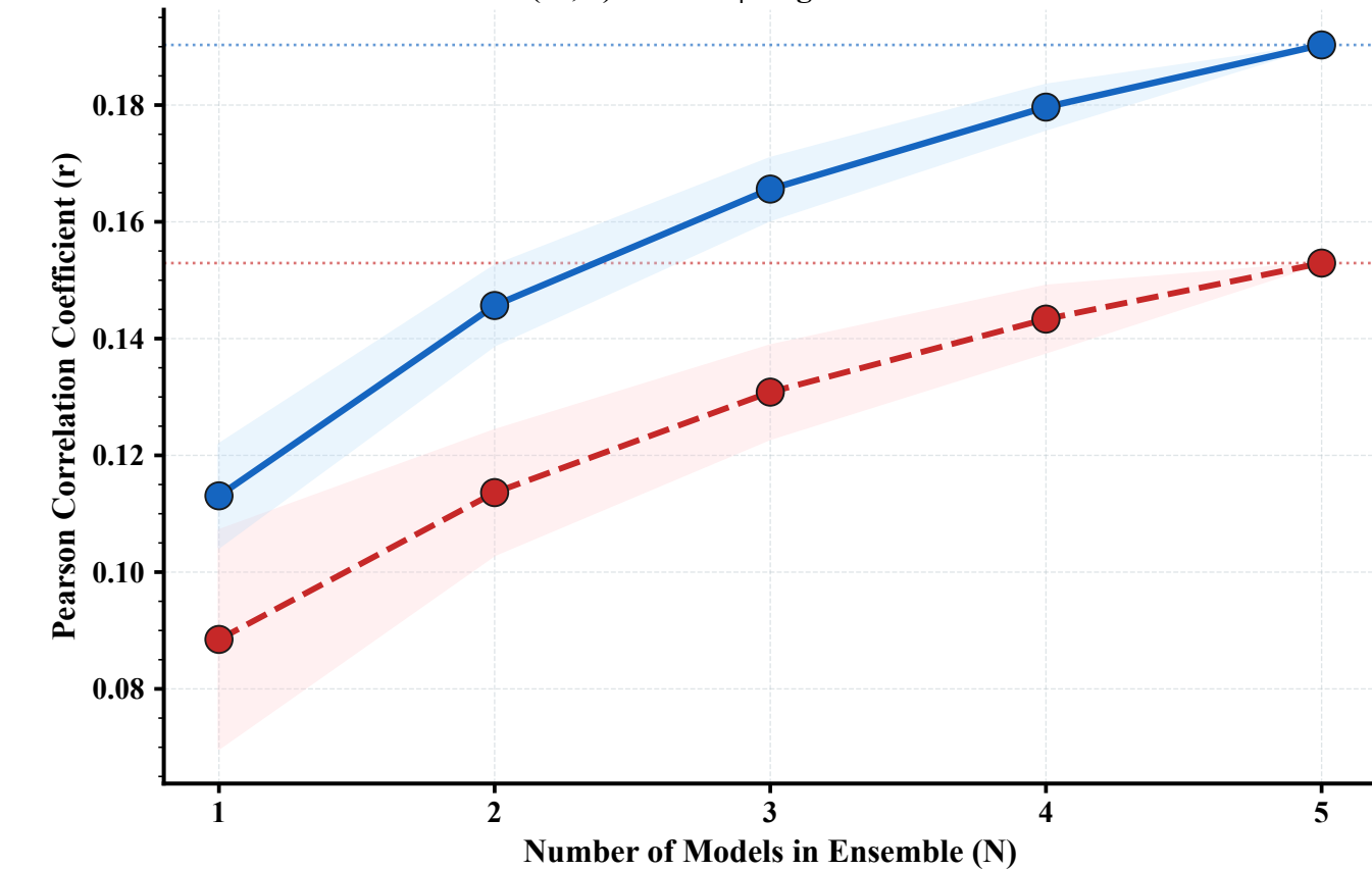
(c) Pearson Correlation Coefficient (r) Mean \pm SD across all C(M,N) subsets | Higher = better
