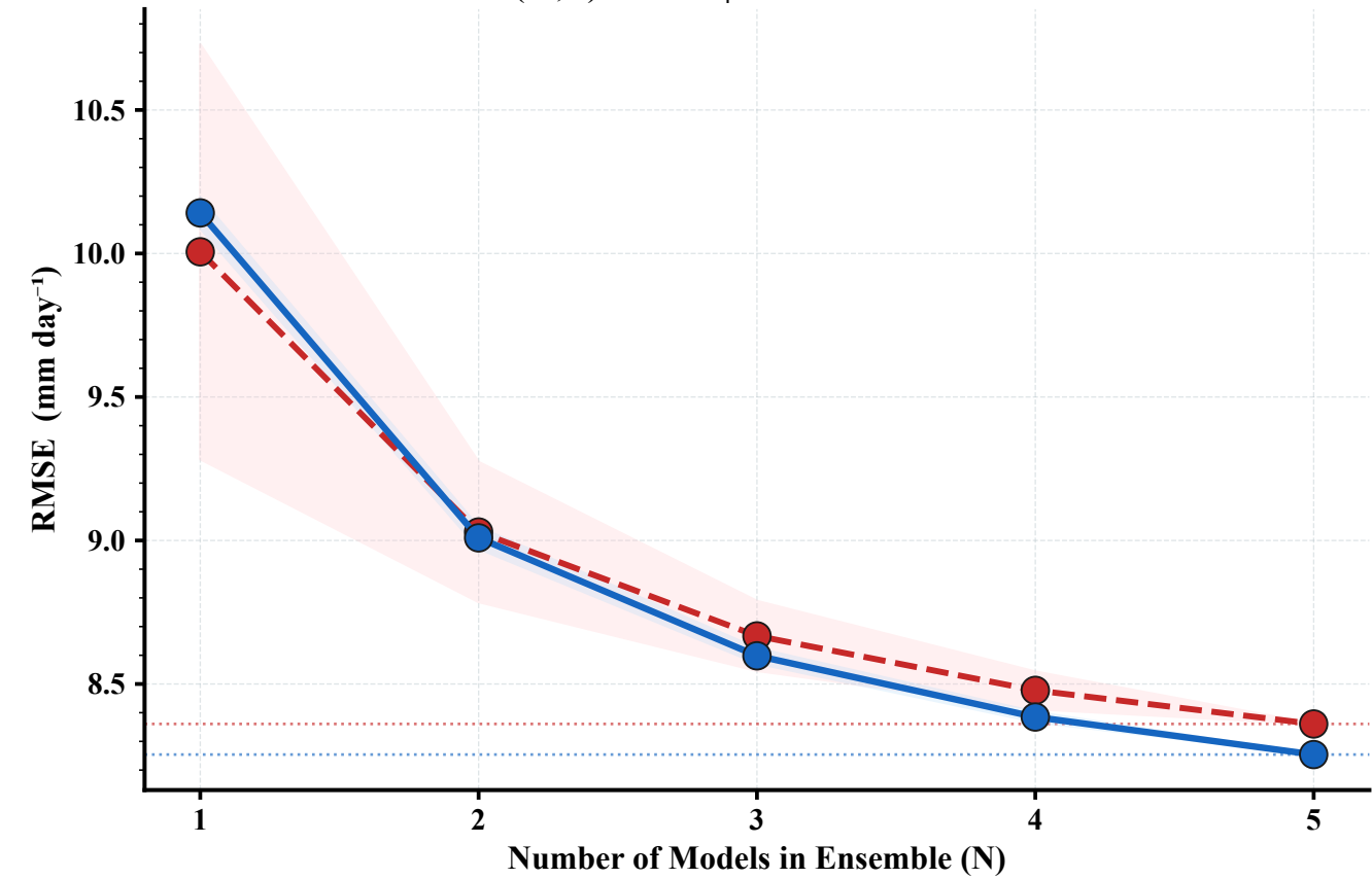
(b) RMSE (mm day -1 ) Mean \pm SD across all C(M,N) subsets | Lower = better
