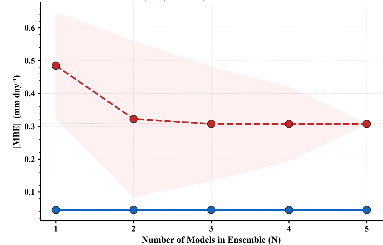
(d) |MBE| (mm day -1 ) Mean \pm SD across all C(M,N) subsets | Closer to 0 = better
